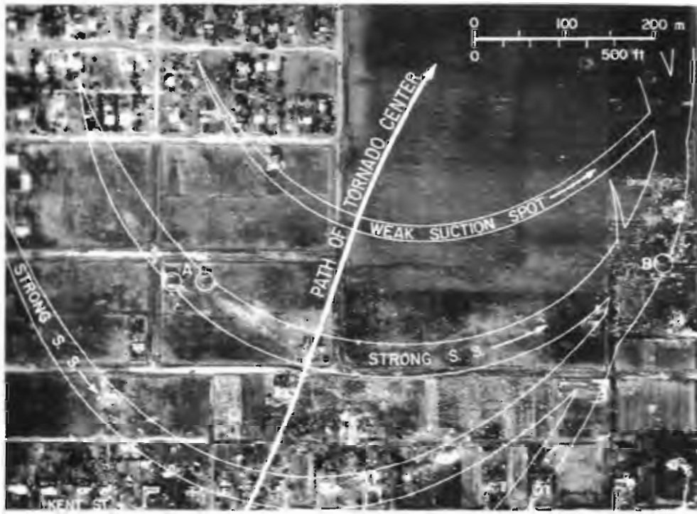
Fig. III. Pattern of three suction swaths north of Kent St. Destructive damage can be followed within each suction swath in the direction of arrows. Note that the extent of damage is not always related to distance of structures from tornado center. (Picture by NASA)
