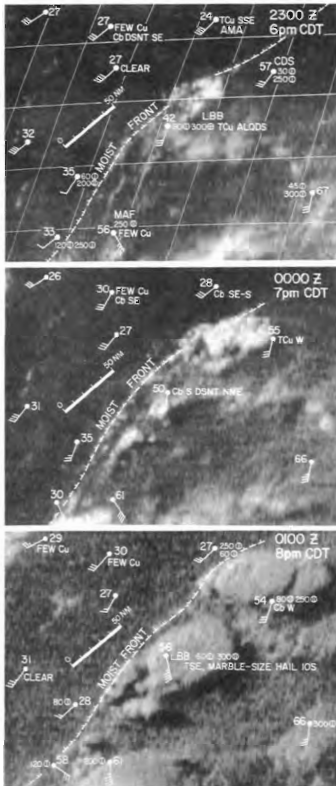
Fig. 8. Three satellite pictures showing the development of the Lubbock meso-scale cloud. Upper picture has a superimposed one degree latitude-longitude grid. The advancing front of moist air from the Gulf is indicated as "moist front." Each wind barb equals 5 knots. (8X enlargement satellite pictures by NASA)
